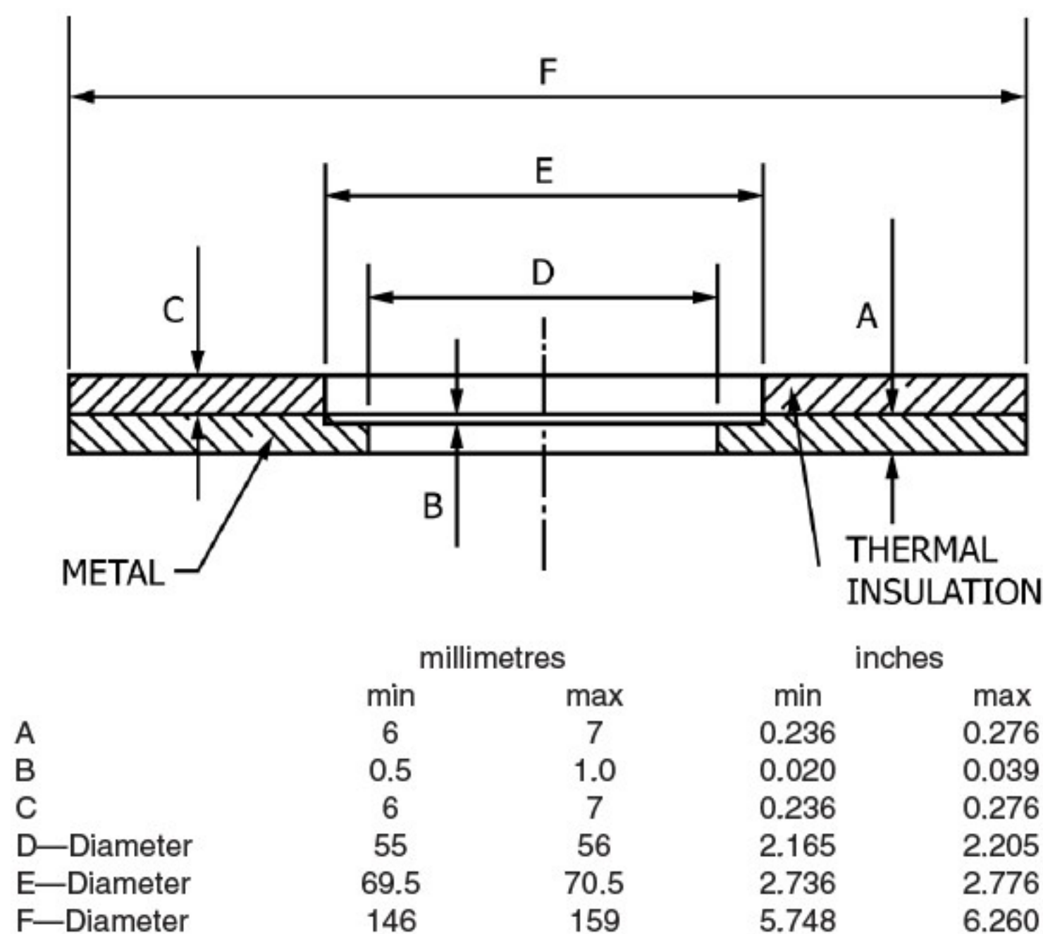
FIG. 2 Heating Plate
